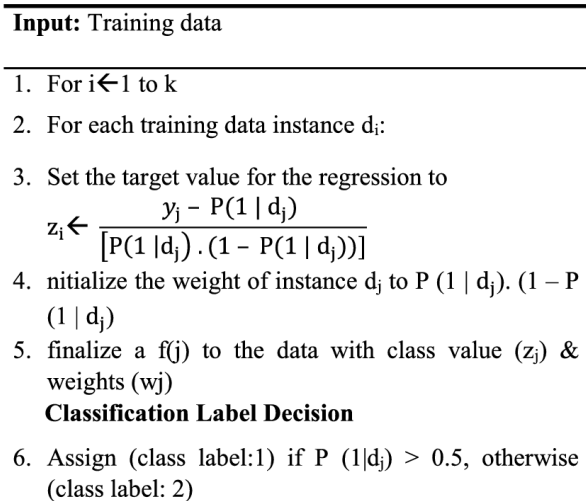
Figure 6: Logistic Regression Algorithm [10]
