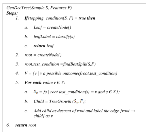
Figure 7: Decision Tree Algorithm [10]
