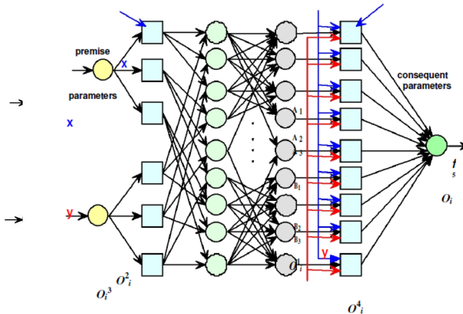
Figure 5. Architecture of the ANFIS
