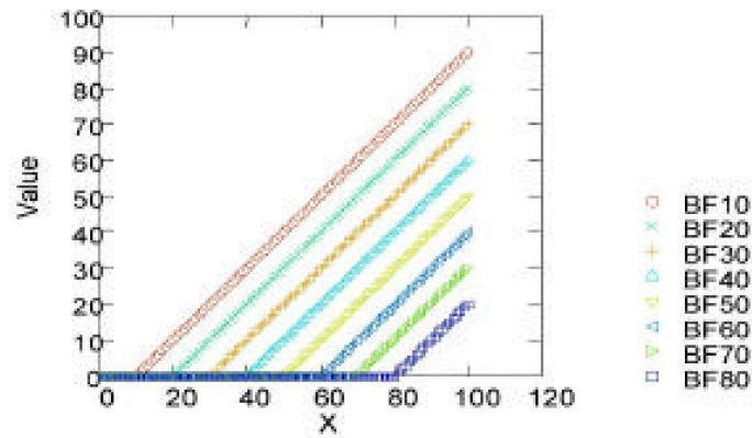
Figure 2. Variations of basis functions for c = 10 to 80
